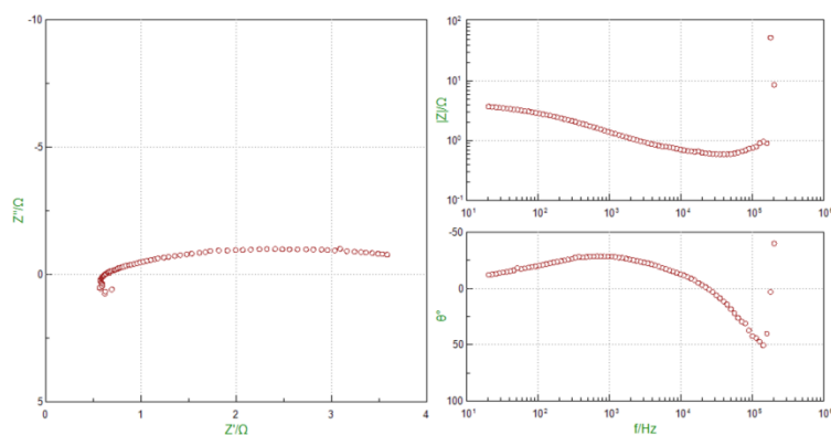
Figure 3.3 EIS Results of the Supercapacitor Electrode at a 10:0 Ratio
