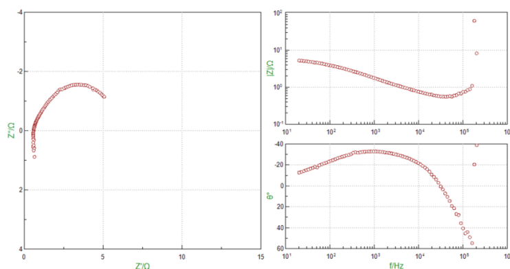
Figure 3.7 EIS Results of the Supercapacitor Electrode at a 0:10
