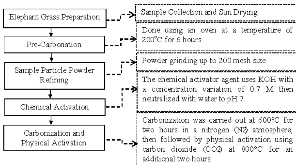
Figure 2.1. Flowchart of activated carbon production from elephant grass
