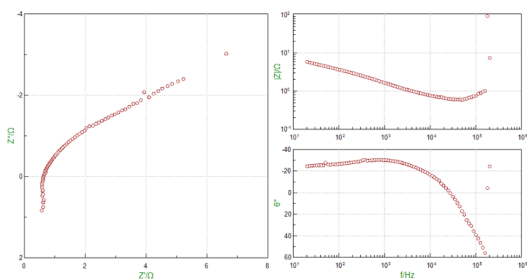
Figure 3.5 EIS Results of the Supercapacitor Electrode at a 05:05 Ratio
