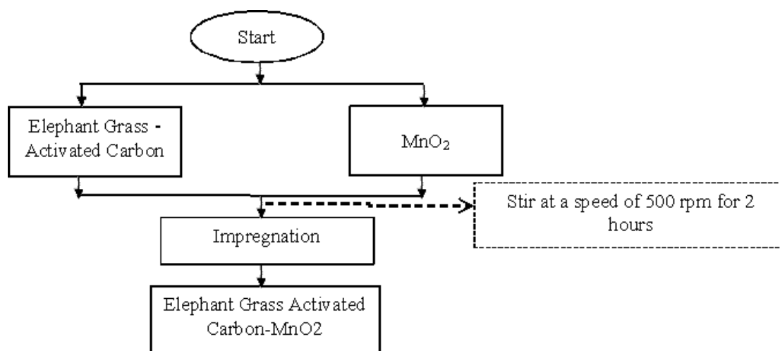
Figure 2.1. Flowchart of activated carbon and manganese dioxide composite fabrication
