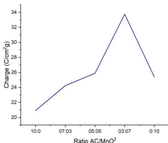
Figure 3.2 Graph of specific charge against the ratio of activated carbon and manganese dioxide
