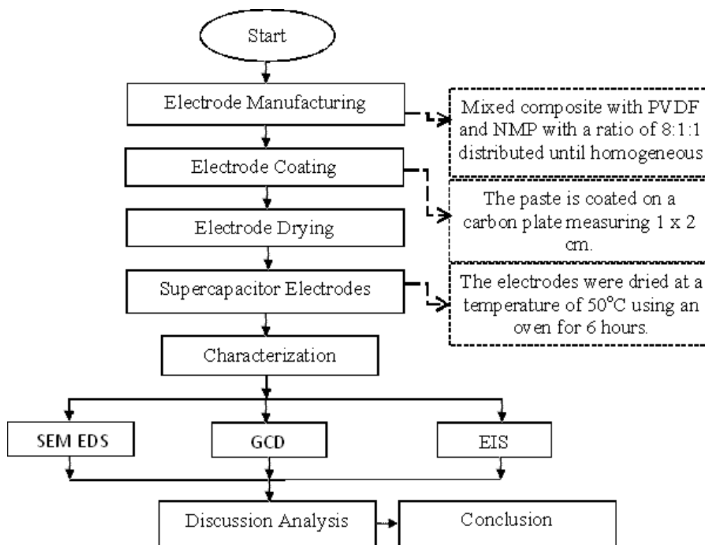
Figure 2.1. Flowchart of supercapacitor electrode fabrication
