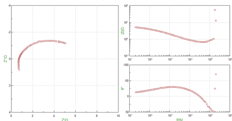
Figure 3.6 EIS Results of the Supercapacitor Electrode at a 07:03 Ratio
