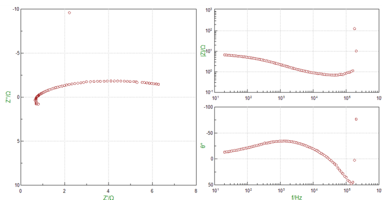
Figure 3.4 EIS Results of the Supercapacitor Electrode at a 07:03 Ratio
